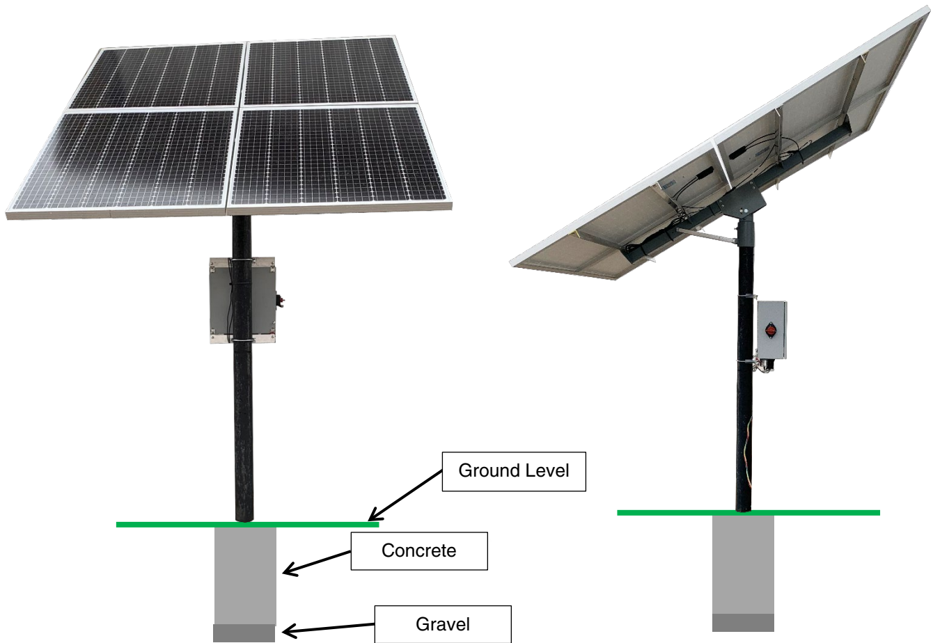
FRONT VIEW
